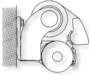
Wall mount dimensions 8 1/2" W x 8 1/2" H
